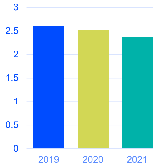
Jordan
