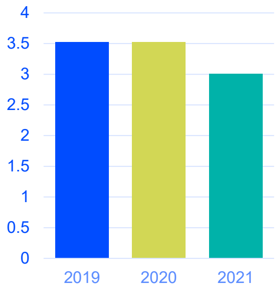
Jordan
